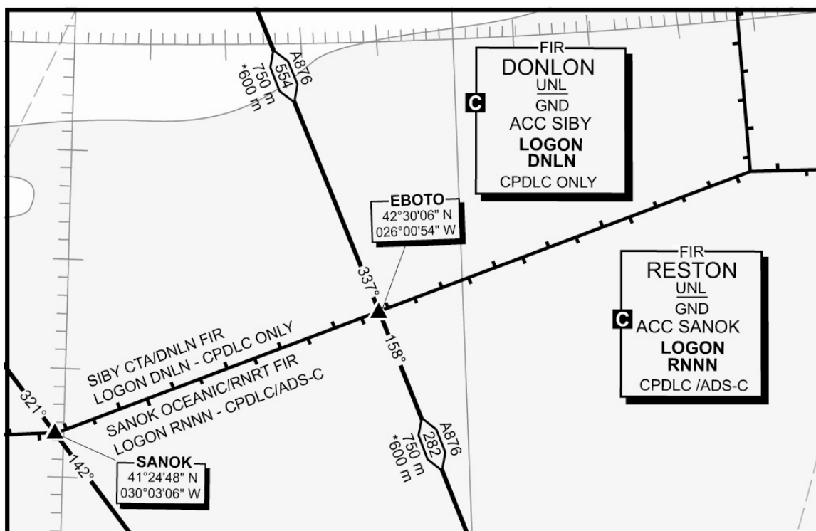
Figure 5-1. FIR designator and CPDLC logon address on en route chart
