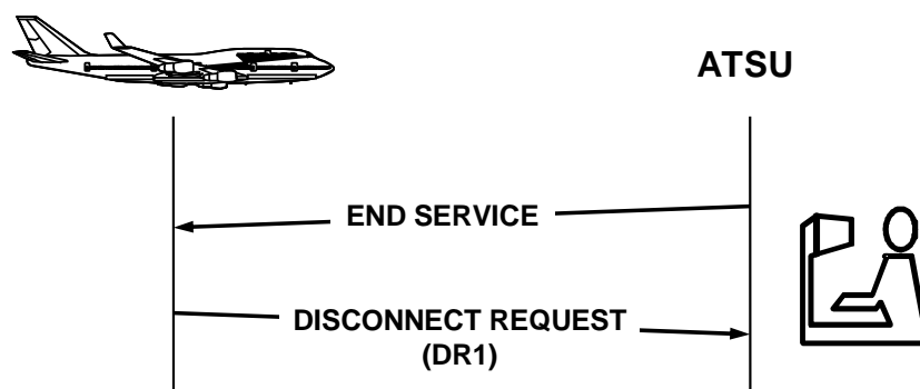
Figure 2-12. Termination of the CPDLC connection
